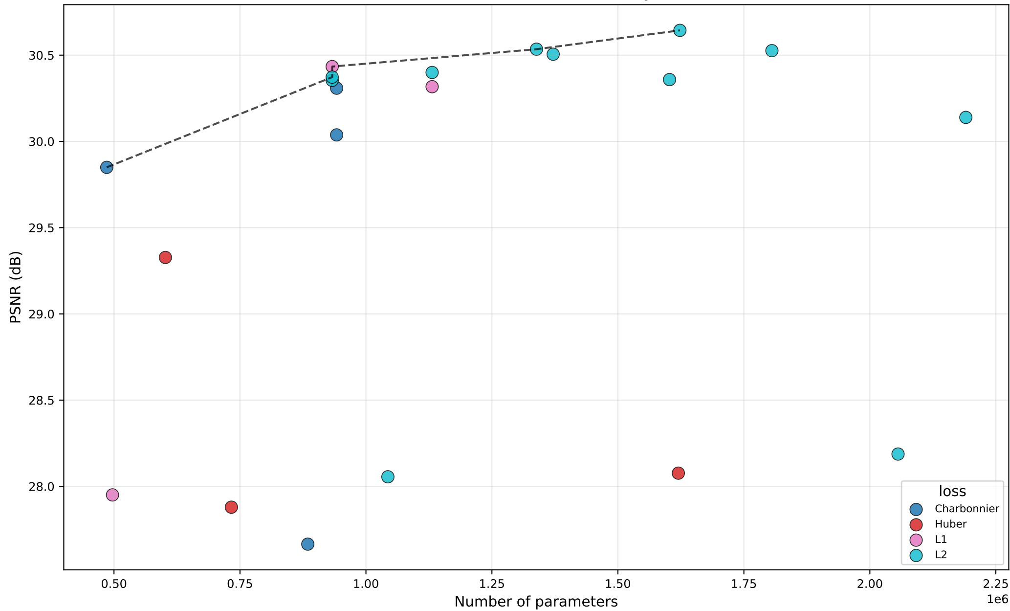
PSNR vs #Params — ELAN — by loss
